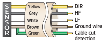
» 5-wires
