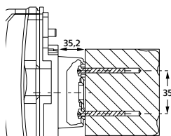
Wall mounting
