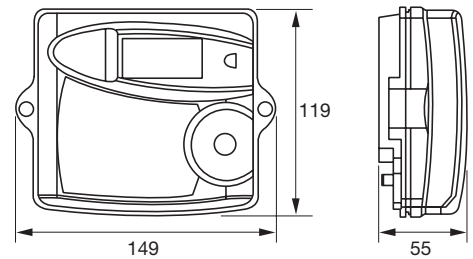
Integrator
